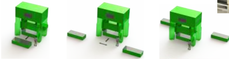
20000 kN Mechanical Transfer Press Big Rapids Products, Kentucky, USA Bolster Size 7600 mm x 2800 mm, 3-Axis Servo Transfer System
